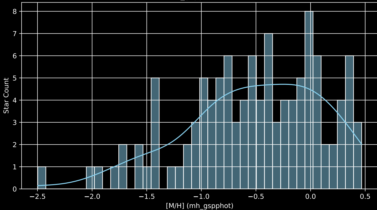
APOGEE DR17 Field: [015+00 [M/H] (mh_gspphot) (n= 112)
