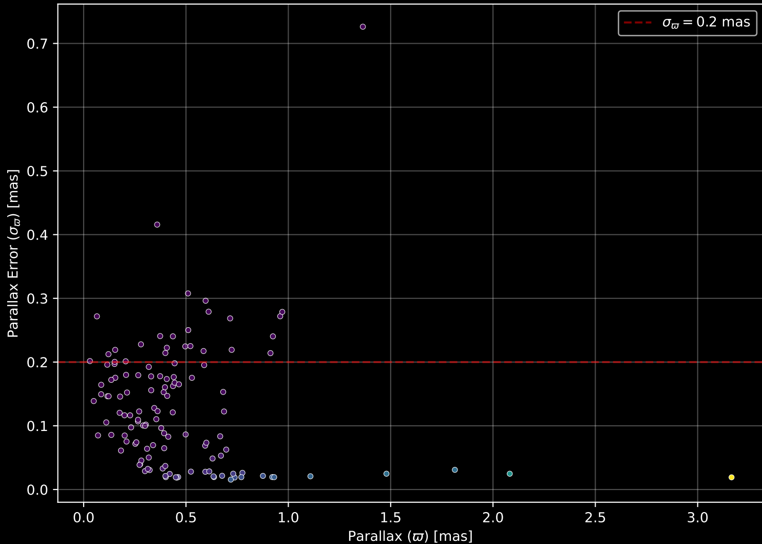
APOGEE DR17 Field: [015+00] Parallax Quality (n= 125)
