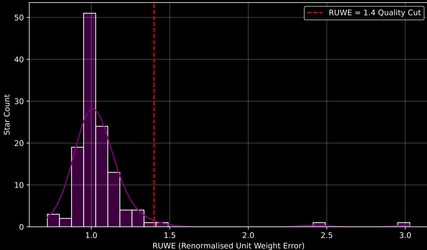
GAPOGEE DR17 Field [015+00] RUWE Distribution (n= 124)
