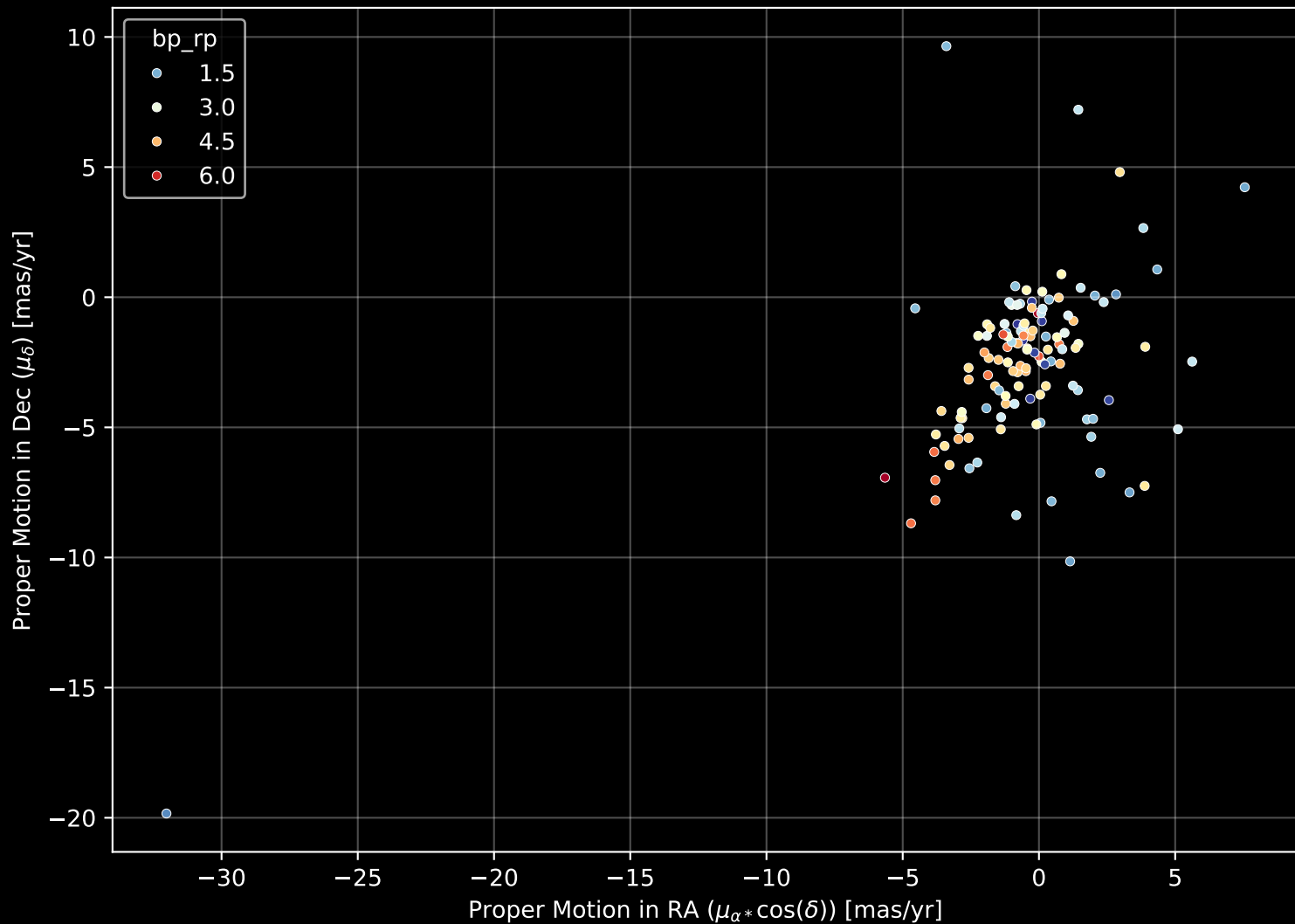
APOGEE DR17 Field: [015+00] Proper Motion Diagram (n= 125)
