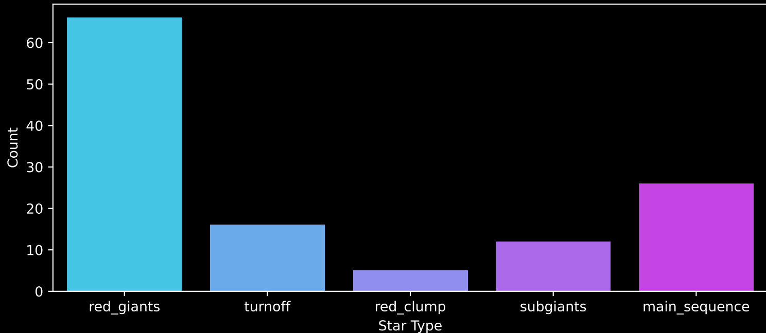
APOGEE DR17 Field: [015+00] Count plot of Star Type
